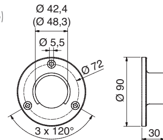
Edelstahl (A2/A4) | stainless steel (304/316)
